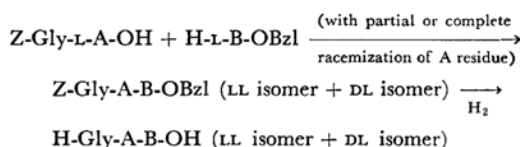
Fig. 1. Supposed sequence of synthesis of tripeptide diastereomers.
