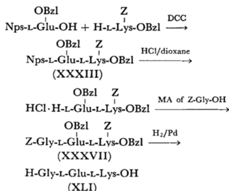
Fig. 3. Sequence of synthesis of tripeptide (XLI). Nps-, o -nitrophenylsulfenyl; DCC, dicyclohexylcarbodiimide.
