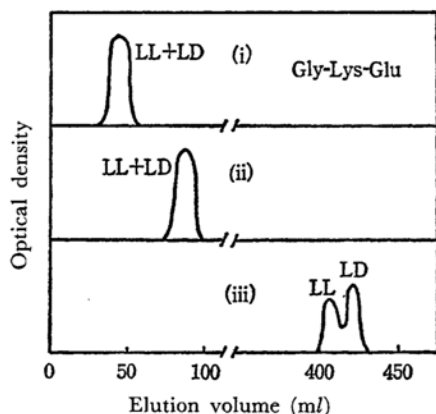
Fig. 6. Elution pattern of a diastereomeric mixture of Gly-Lys-Glu. (i), (ii) and (iii); see Fig. 5.
