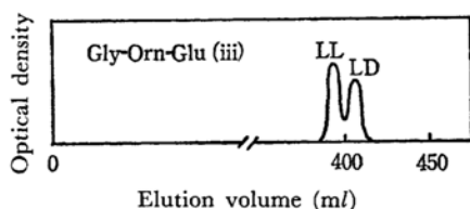
Fig. 7. Elution pattern of a diastereomeric mixture of Gly-Orn-Glu. (iii); see Fig. 5.
