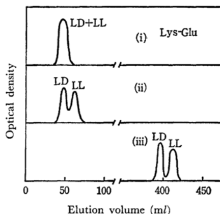
Fig. 5. Elution pattern of a diastereomeric mixture of Lys-Glu.
