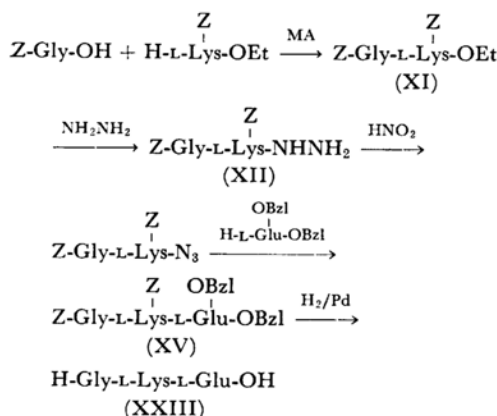
Fig. 2. Sequence of synthesis of tripeptide (XXIII).
