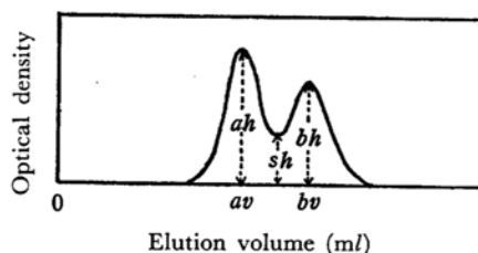
Fig. 4. Model elution pattern of a diastereomeric mixture.
